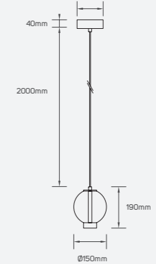
● 661688 6W ■ Metal + Glass IP 20 CRI 80 □ AC220-240V
