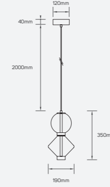
● 661687 10W ■ Metal + Glass IP 20 CRI 80 □ AC220-240V
