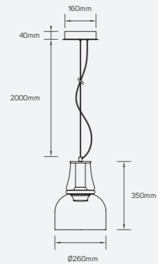
● 661684 14W ■ Metal + Glass IP 20 CRI 80 □ AC220-240V
