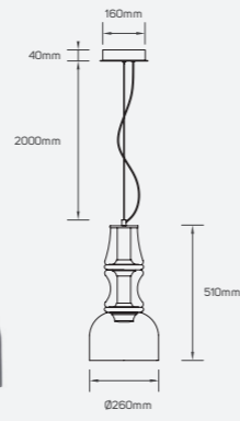
● 661685 23W ■ Metal + Glass IP 20 CRI 80 □ AC220-240V
