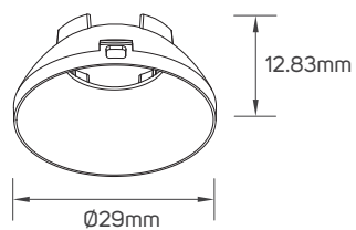
● 613513 - ● 613514 - ● 613515 - ● 613516 - Reflector
