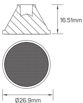
613540 - Lens
