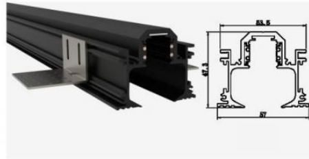
Size:53.5X47.3X57mm
