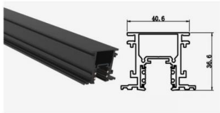
Size:40.6X36.6X48.8mm
