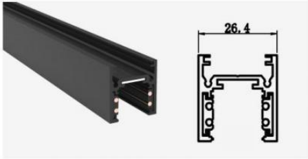
Size:26.4X26.4X26.4mm
