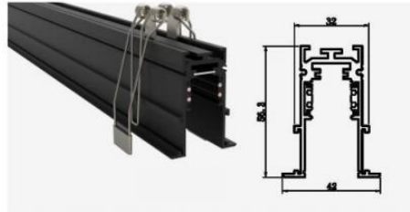
Size:32X56.3X42mm
