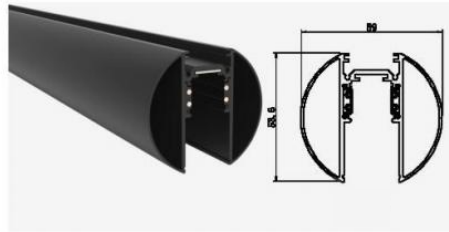
Size:59X53.6X59mm
