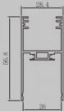
Surface mounted / lifting track
