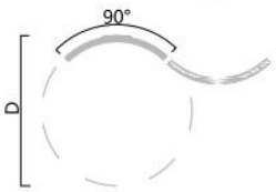
90 degree arc track combination Sizes of diameter D: 60cm, 90cm, 120cm, 200cm, 250cm, 300cm, 350cm.
