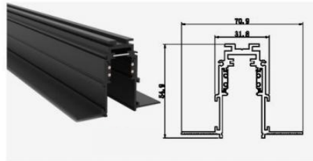
Size:70.9X54.9X31.8mm
