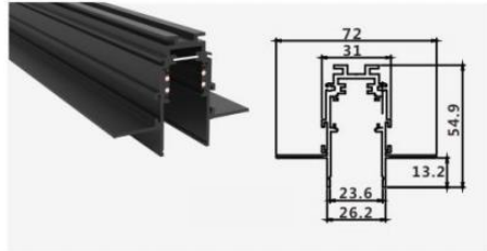
Size:31X53X72mm
