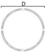
Round track combination Sizes of diameter D: 60cm, 90cm, 120cm, 200cm, 250cm, 300cm, 350cm.
