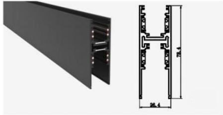
Size:26.4X78.4X26.4mm
