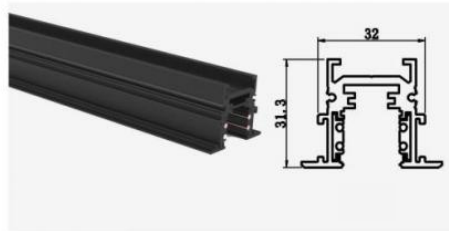
Size:31.3X32X42mm
